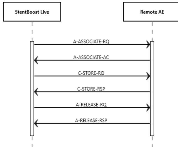
Figure 4: Data Flow Diagram – Store Image – Storage as SCU
