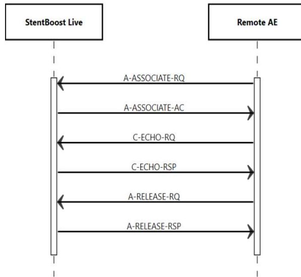
Figure 6: Data Flow Diagram – Verification as SCP
