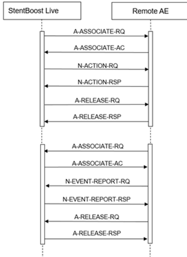
Figure 5: Data Flow Diagram -Storage Commitment as SCU
